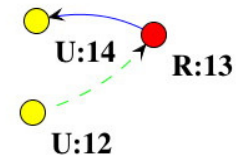
Figure 2: An associogram.
