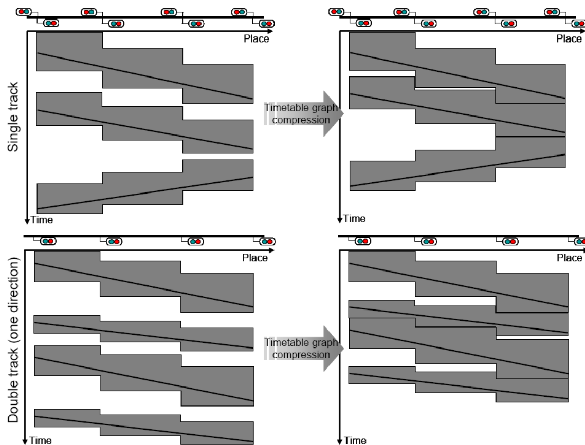
Figure 1: Compression of timetable graph according to the UIC406 capacity method. Partly based on [10].
